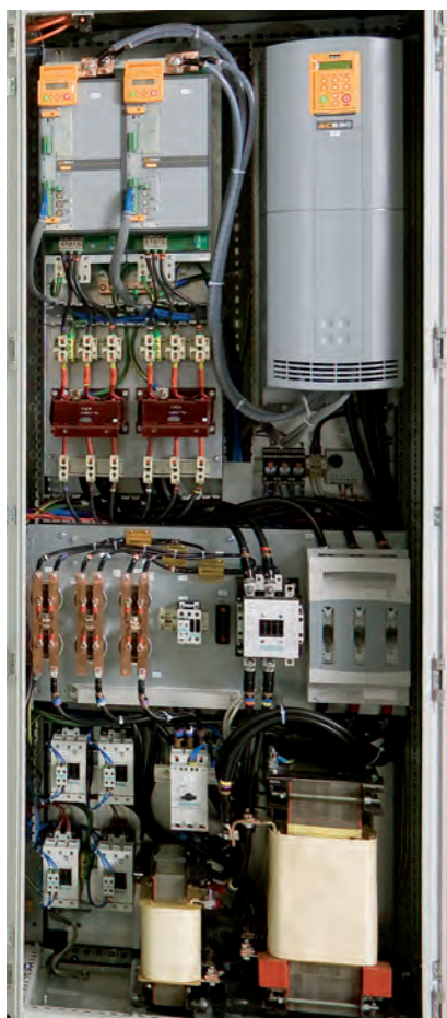
Image shows a typical 4 Quadrant system implemented using AC890 Modular Systems Drives
